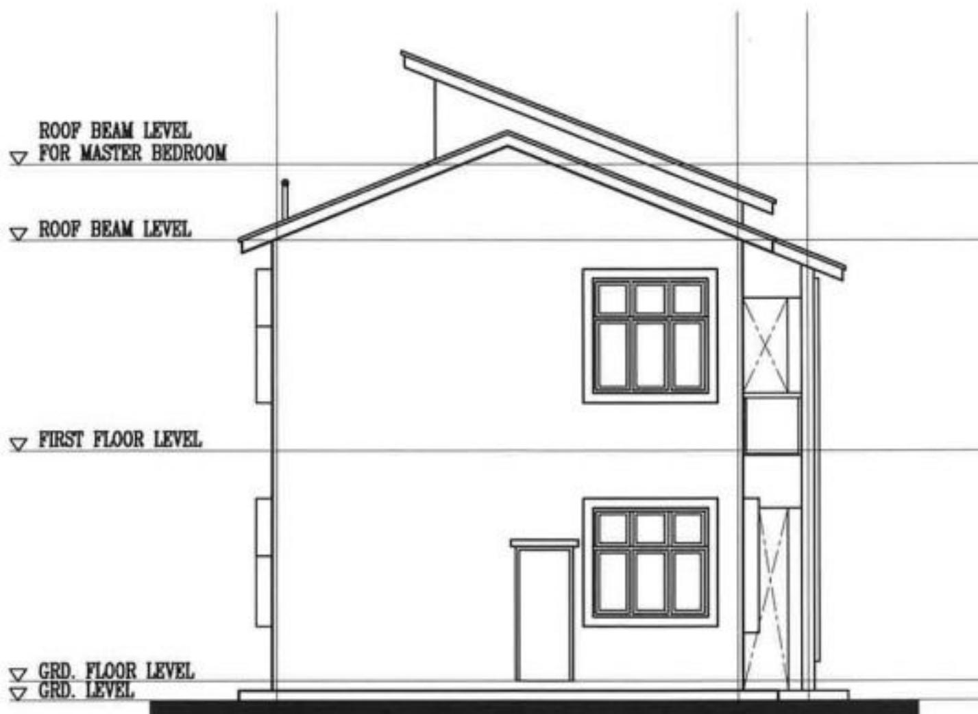
REAR ELEVATION
